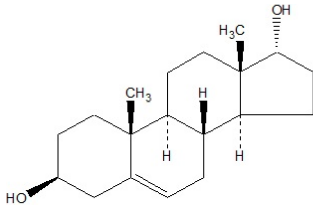
5-Androsten-3beta, 17alpha-diol
